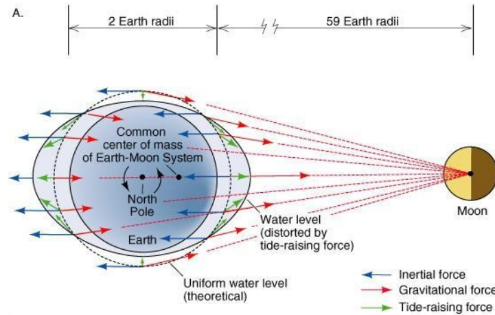
FIGURE 18. Tidal forces
