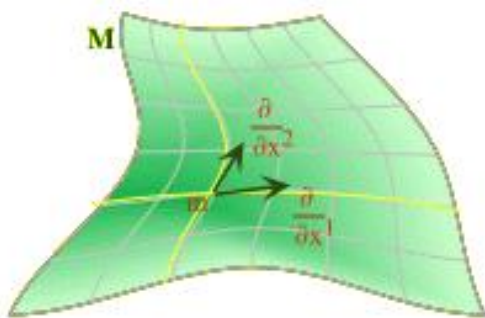
FIGURE 15. Line element
