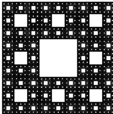
Figure 1: The Sierpinski carpet.
