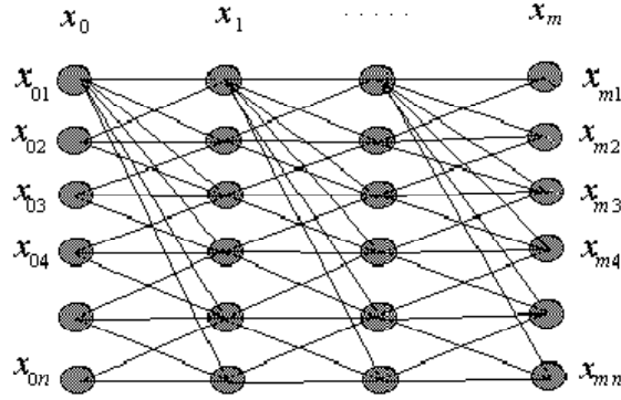
Fig. 1: A multilayer neural network with m = 4 layers; feedforward connections completely connect each layer to the next. Input is x_0 and output is x_m .
