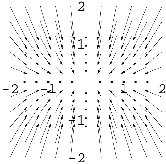
Scaled Vector Field A
