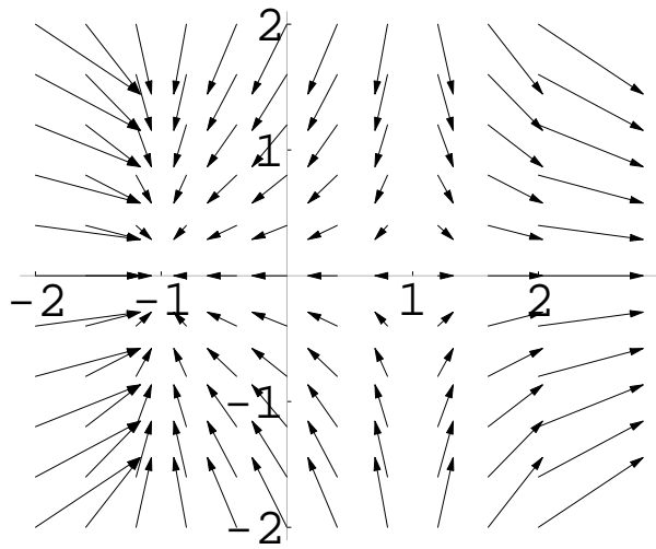
Scaled Vector Field B
