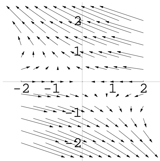
Scaled Vector Field D
