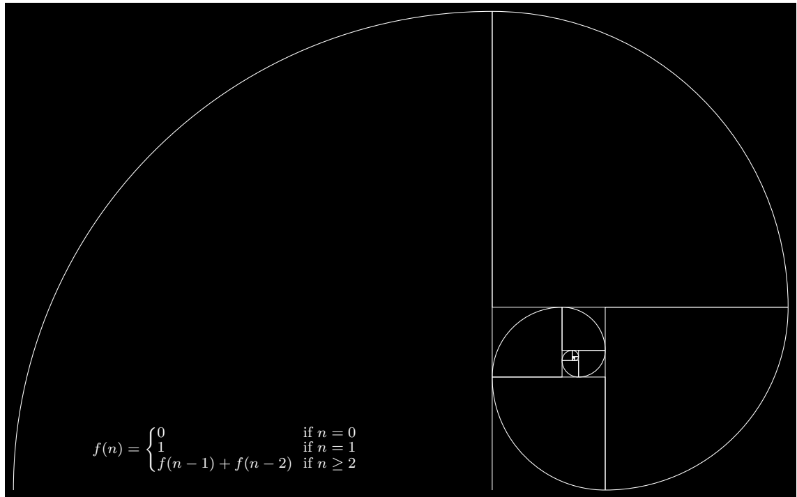
Fibonacci spiral - Author: Andrew Mertz
